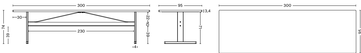
PASSERELLE TABLE | LINOLEUM | LAMINATE TABLETOP WIDTH 300 CM | 118" DEPTH 95 CM | 37.5" HEIGHT 74 CM | 29.25" CROSSBAR HEIGHT 39 CM | 15.5"
