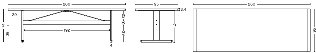
PASSERELLE TABLE | VENEER TABLETOP WIDTH 260 CM | 102.5" DEPTH 95 CM | 37.5" HEIGHT 74 CM | 29.25" CROSSBAR HEIGHT 39 CM | 15.5"
