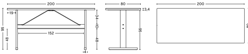
PASSERELLE HIGH TABLE | LINOLEUM | LAMINATE TABLETOP WIDTH 200 CM | 78.75" DEPTH 80 CM | 31.5" HEIGHT 95 CM | 37.5" CROSSBAR HEIGHT 48 CM | 19"
