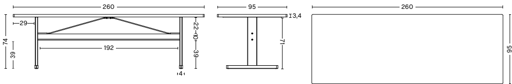
PASSERELLE TABLE | LINOLEUM | LAMINATE TABLETOP WIDTH 260 CM | 102.5" DEPTH 95 CM | 37.5" HEIGHT 74 CM | 29.25" CROSSBAR HEIGHT 39 CM | 15.5"
