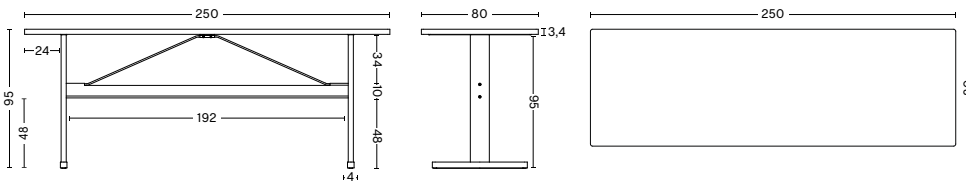
PASSERELLE HIGH TABLE | LINOLEUM | LAMINATE TABLETOP WIDTH 250 CM | 98.5" DEPTH 80 CM | 31.5" HEIGHT 95 CM | 37.5" CROSSBAR HEIGHT 48 CM | 19"
