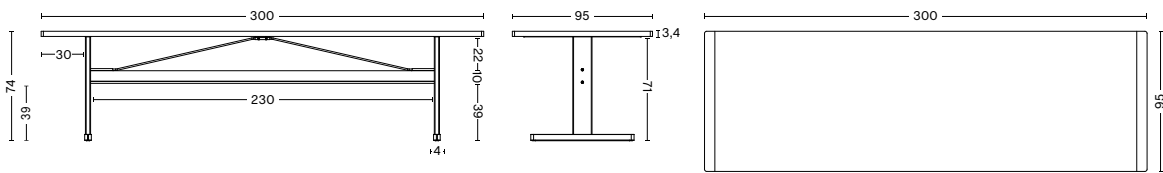
PASSERELLE TABLE | VENEER TABLETOP WIDTH 300 CM | 118" DEPTH 95 CM | 37.5" HEIGHT 74 CM | 29.25" CROSSBAR HEIGHT 39 CM | 15.5"
