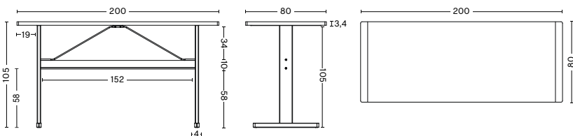
PASSERELLE HIGH TABLE | VENEER TABLETOP WIDTH 200 CM | 78.75" DEPTH 80 CM | 31.5" HEIGHT 105 CM | 41.25" CROSSBAR HEIGHT 58 CM | 22.75"
