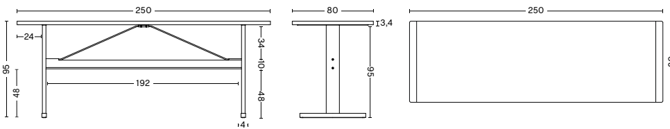
PASSERELLE HIGH TABLE | VENEER TABLETOP WIDTH 250 CM | 98.5" DEPTH 80 CM | 31.5" HEIGHT 95 CM | 37.5" CROSSBAR HEIGHT 48 CM | 19"
