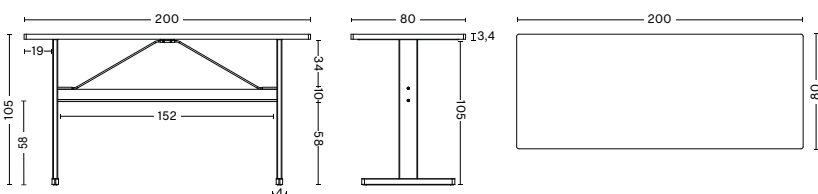
PASSERELLE HIGH TABLE | LINOLEUM | LAMINATE TABLETOP WIDTH 200 CM | 78.75" DEPTH 80 CM | 31.5" HEIGHT 105 CM | 41.25" CROSSBAR HEIGHT 58 CM | 22.75"
