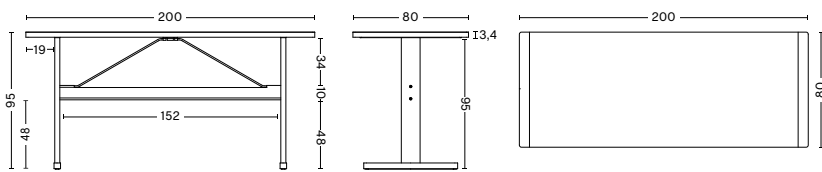
PASSERELLE HIGH TABLE | VENEER TABLETOP WIDTH 200 CM | 78.75" DEPTH 80 CM | 31.5" HEIGHT 95 CM | 37.5" CROSSBAR HEIGHT 48 CM | 19"
